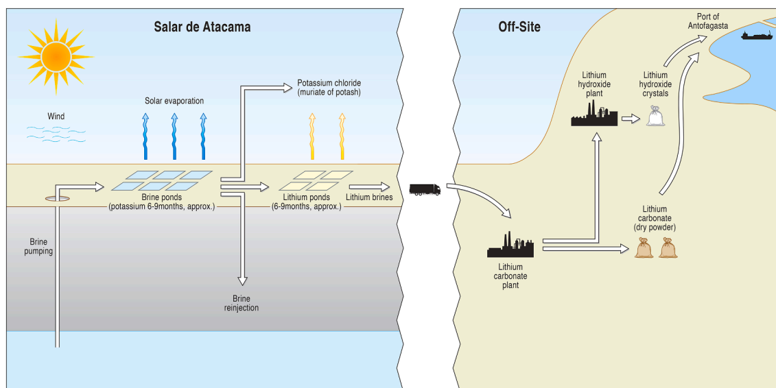
Fig. 2. The lithium-from-brine process on the Salar de Atacama.
