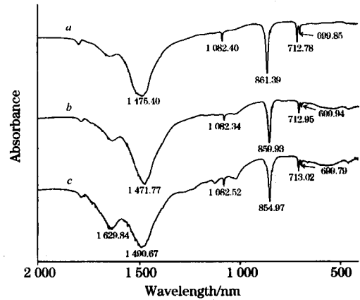
Fig. 3 Typical FTIR spectra of aragonites in the range of 500\sim 2\,000\text{ cm}^{-1}
