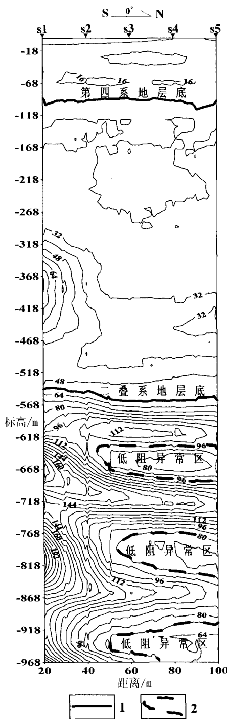
图4 测线 1 视电阻率等值断面解释图 Fig. 4 Comparatively apparent resistivity equivalence section of Line 1 1—地层界线;2—异常区 1—Stratigraphic boundary; 2—Abnormal region
