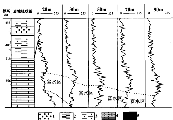
图3 刘桥二矿 II617 工作面测线 1 富水区解释图 Fig. 3 Water - rich area interpretation of curves on Line 1.
