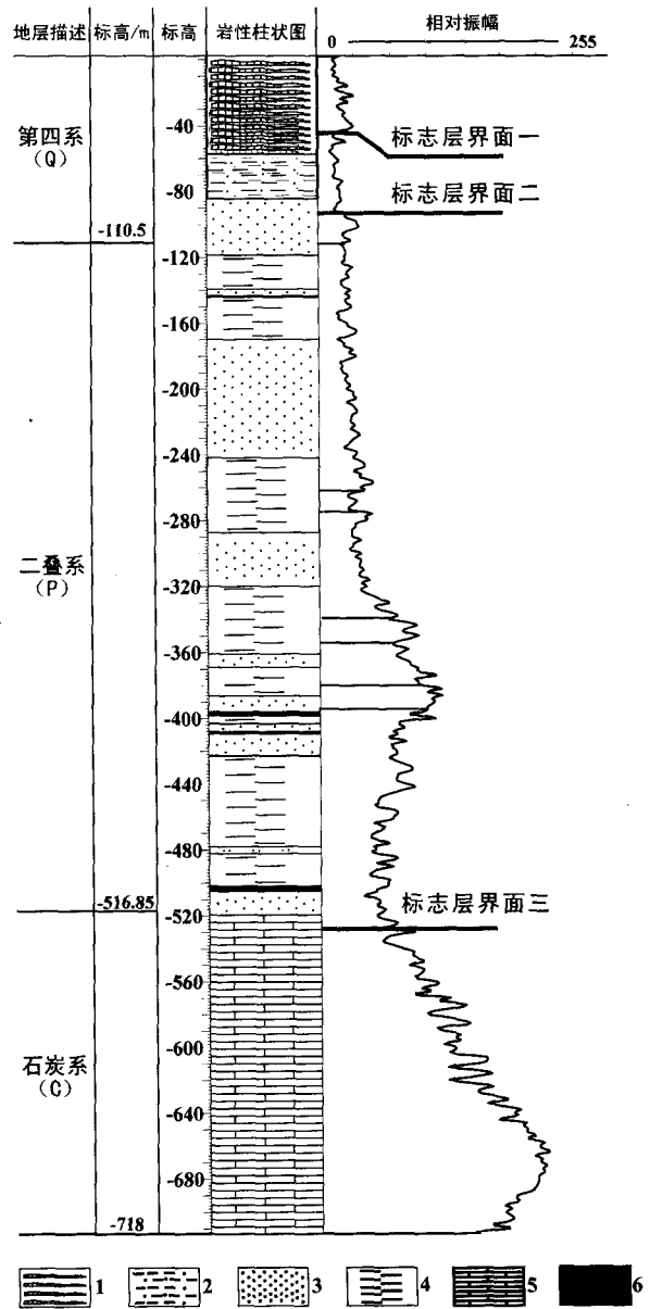
图2 测线1测点01测深曲线地质界面解释图 Fig.2 Geological interpretation of curves at Point 01 on Line 1
