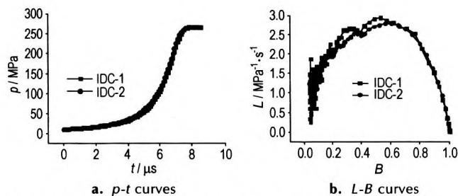
Fig. 2 p-t Curves and L-B curves for two kinds of propellants
