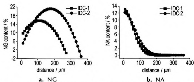
Fig. 1 Concentration profiles of NG and NA in two kinds of propellants
