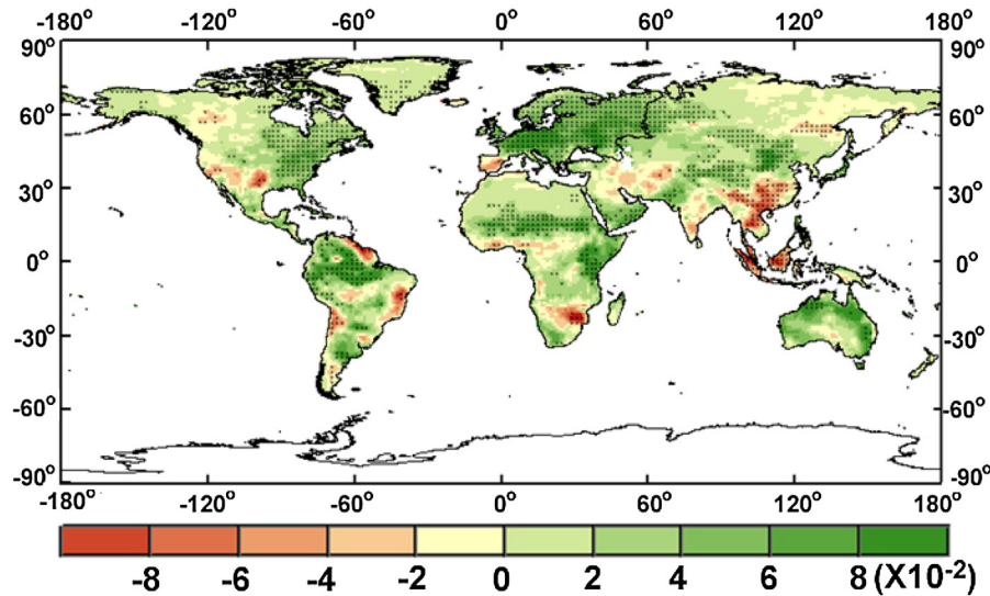
Fig. 12. Map of the linear trend in the merged LE based on the BMA method driven by seven CMIP5 GCM datasets during 1970–2005. The solid dots refer to grids with 95% confidence. Unit: \text{W/m}^2 per year.
