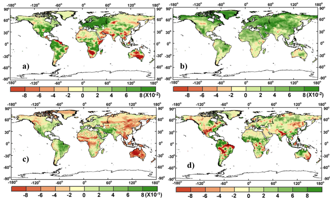
Fig. 13. Maps of the linear trends in the merged (a) LE based on the BMA method driven by seven CMIP5 GCM datasets (Unit: \text{W/m}^2 per year), (b) T_a from ERA-Interim (Unit: ^{\circ}\text{C} per year), (c) R_s from GEWEX (Unit: \text{W/m}^2 per year) and (d) P from PGF (Unit: mm per year) during 1984–2005. The solid dots refer to grids with 95% confidence.
