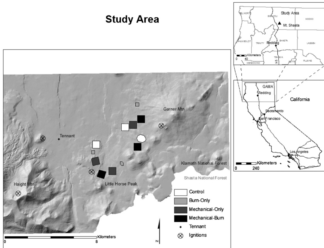
Fig. 1. Location of study area, the town of Tennant, and the four ignition points for the landscape fire simulations.
