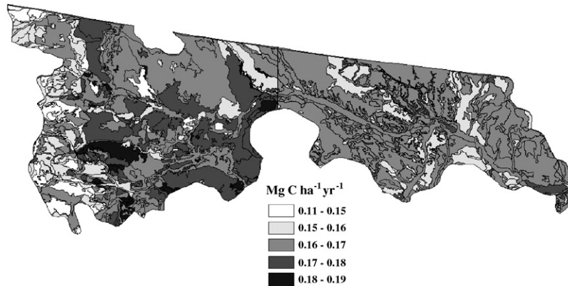
Fig. 8. Soil C change rates predicted by the Century model in an example area in Montana in no-tillage fallow-small grain rotations, plotted by the intersection of soil type, land use, native vegetation and climate region.
