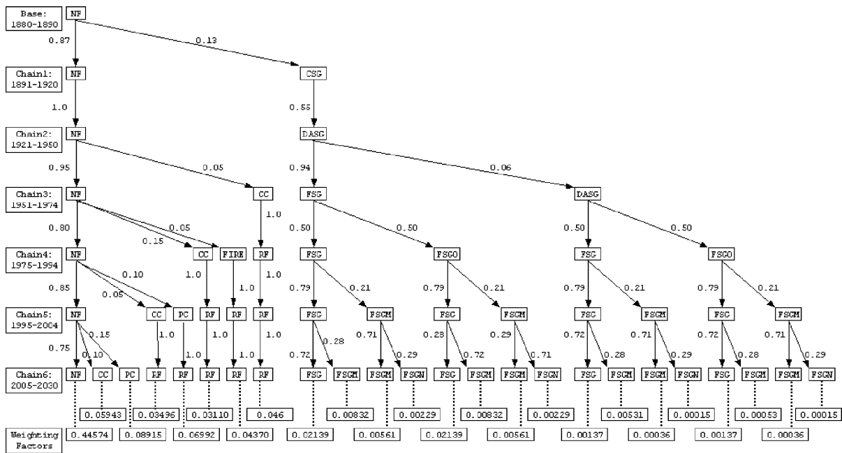
Fig. 6. Management sequence diagram for Major Land Resource Area 46. N.B.: NF, native forest; CC, clear cut tree removal; PC, partial cut tree removal; FIRE, stand-replacing fire; RF, regenerating forest; CSG, continuous small grains; DASC, dryland alfalfa-small grain; FSG, fallow-small grain (conventional tillage); FSGO, fallow-small grain-oilseed; FSGM, fallow-small grain (minimum tillage); FSGN, fallow-small grain (no tillage). Land management system descriptions and transition rate data are from Paustian et al. (in preparation).
