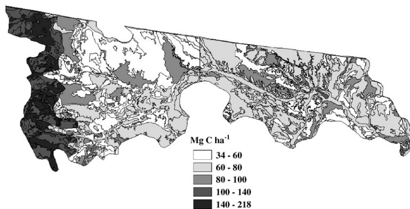
Fig. 7. Soil C stocks predicted by the Century model in an example area in Montana, plotted by the intersection of soil type, land use, native vegetation and climate region.
