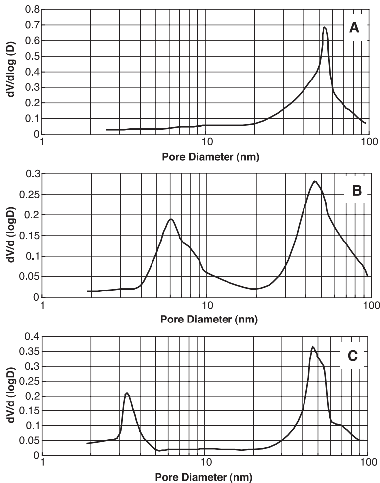
Fig. 1. The pore size distributions of Q-50 and the bimodal pore supports (A) Q-50. (B) Silica bimodal pore support. (C) Zirconia bimodal pore support. (B) The weight ratio of silica from silica sol to Q-50 silica was 11.2%. (C) The weight ratio of zirconia from zirconia sol to Q-50 silica was 16.8%.
