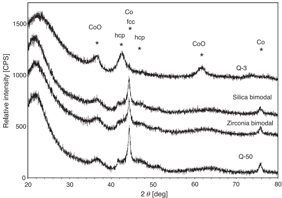
Fig. 4. The XRD patterns of various catalysts. SiO 2 bimodal: The weight ratio of silica from silica sol to Q-50 silica was 11.2%. ZrO 2 bimodal: The weight ratio of zirconia from zirconia sol to Q-50 silica was 16.8%.
