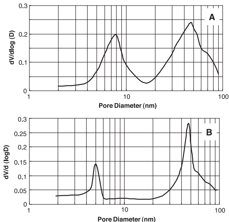
Fig. 5. The pore size distribution of bimodal pore catalysts with Co loading of 10 wt.%. (A) SiO 2 bimodal; the weight ratio of silica from silica sol to Q-50 silica was 11.2%. (B) ZrO 2 bimodal; the weight ratio of zirconia from zirconia sol to Q-50 silica was 16.8%.
