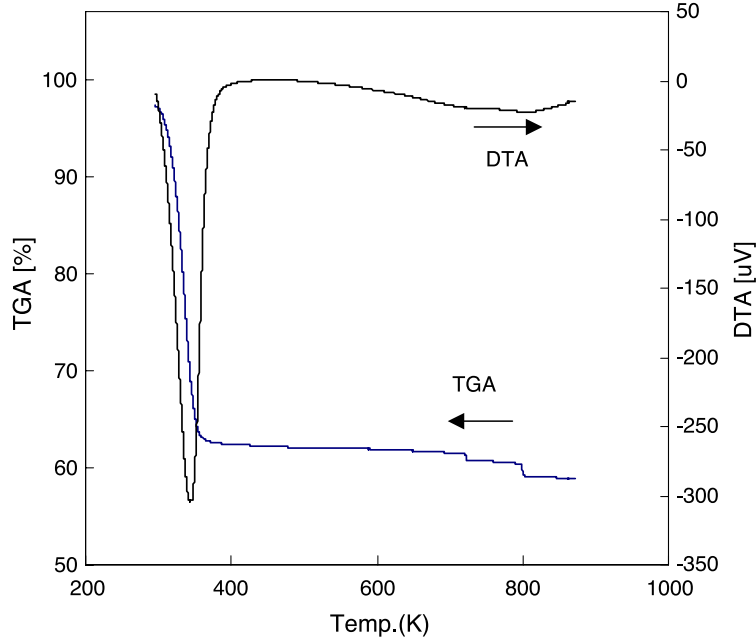
Fig. 3. The TG and DTA profiles of silica bimodal pore support sample. The weight ratio of silica from silica sols to Q-50 silica was 11.2%.
