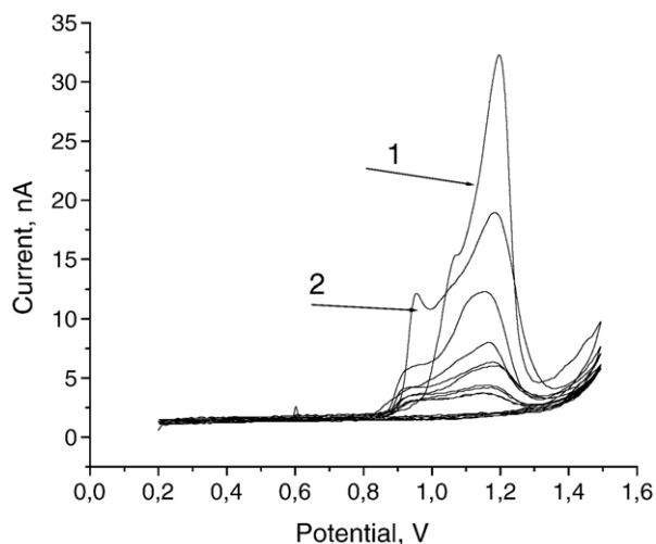
Fig. 3. Cyclic voltamperogramme of electrochemical synthesis of poly(3,4-ethylenedioxythiophene) in 0.02 M phosphate buffer, pH 6.2, involute speed 0.1 V/s, 1, 2 are cycle numbers.
