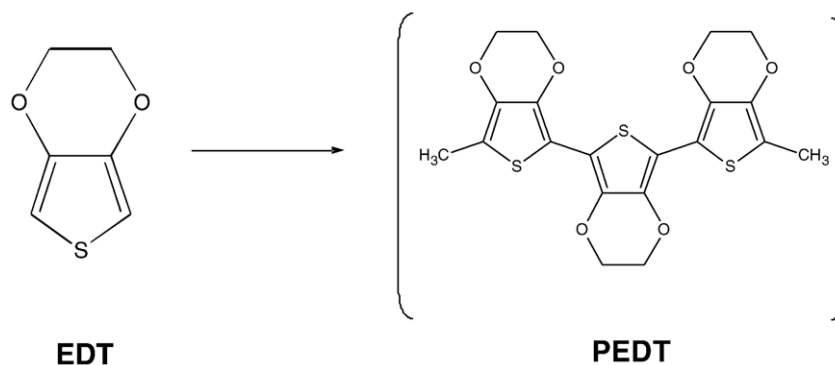
Fig. 1. Basic scheme of PEDT polymerization [23].
