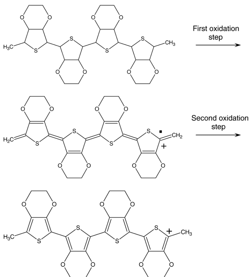
Fig. 2. Suggested mechanism of modification of PEDT structure at electrochemical polymerization [24].
