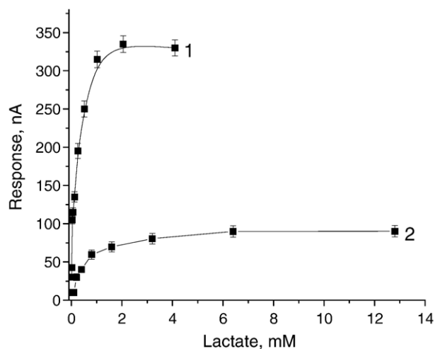
Fig. 6. Calibration curve of amperometric biosensor based on platinum printed SensLab electrode with LOX immobilized in Resydrol by physical adsorption (1) and in PEDT by electrochemical polymerization (2). Measurements were carried out in 100 mM phosphate buffer, pH 7.2, potential +300 mV with regard to internal reference electrode.
