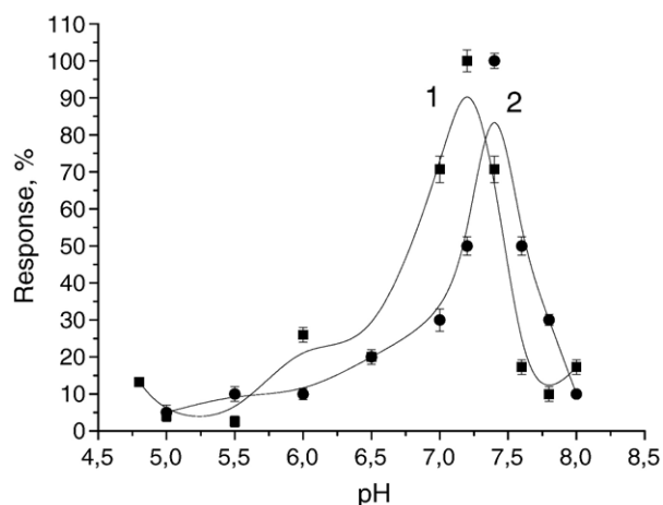
Fig. 4. Response dependence for amperometric biosensors based on lactate oxidase immobilized in Resydrol polymer by physical adsorption (1) and in PEDT polymer by electrochemical polymerization (2) on pH of solution. Measurement was carried out in 100 mM phosphate buffer, pH 7.2, potential +300 mV with regard to internal reference electrode.
