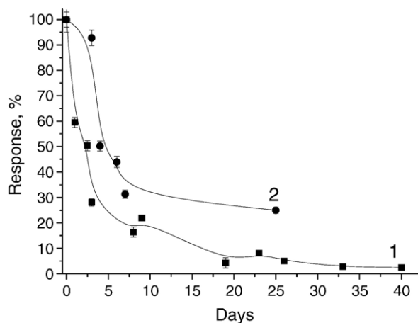
Fig. 5. Stability of amperometric biosensors based on LOX immobilized in Resydrol (1) and in PEDT by electrochemical polymerization (2). Measurement was carried out in 100 mM phosphate buffer, pH 7.2, potential +300 mV with regard to internal reference electrode.
